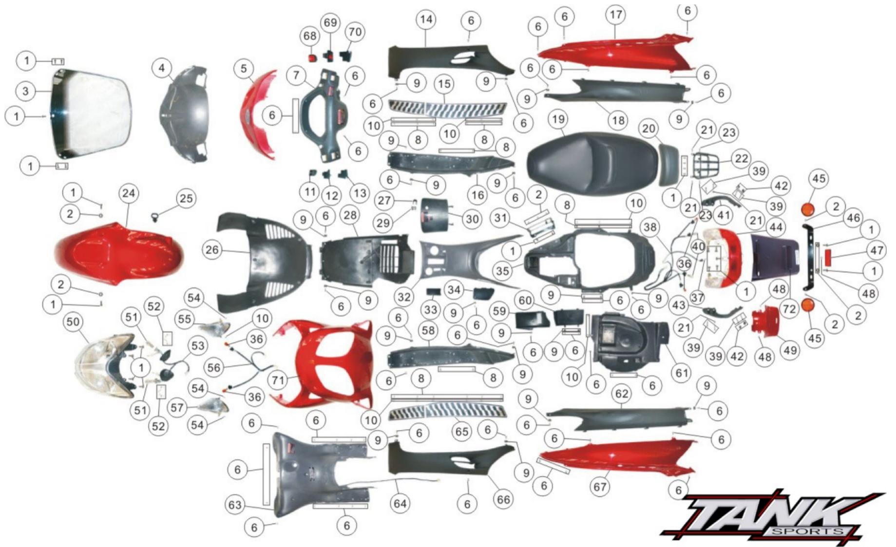
Touring 150 DE Diagram 4 ---- Body & Plastics
